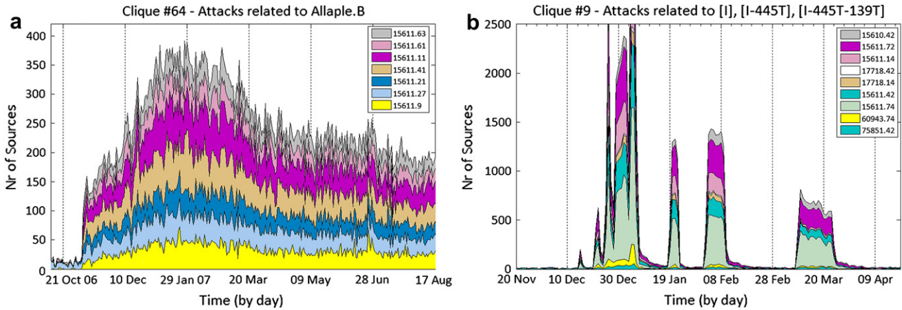
Fig. 3 – (Left) Example of continuous activity: those time series belong to a clique of attacks related W32/Allaple.B on seven different sensors (port sequences: |, |I|139T and |I|139T|445T). (Right) Example of sustained bursts: these time series belong to a clique of attacks related to attack activities on three different sensors, targeting |, |I|445T, |I|445T|139T and |I|445T|80T.
